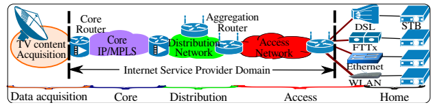
(a) Traditional IPTV architecture
